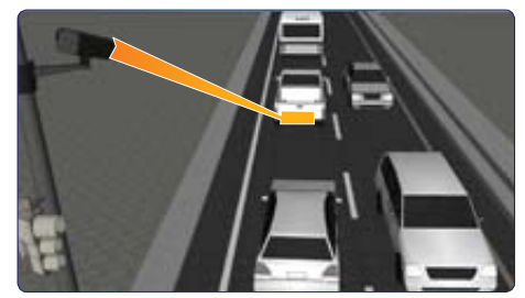
ANPR-40 Camera 10-40mm varifocal lens
