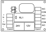
Toggle Relay
